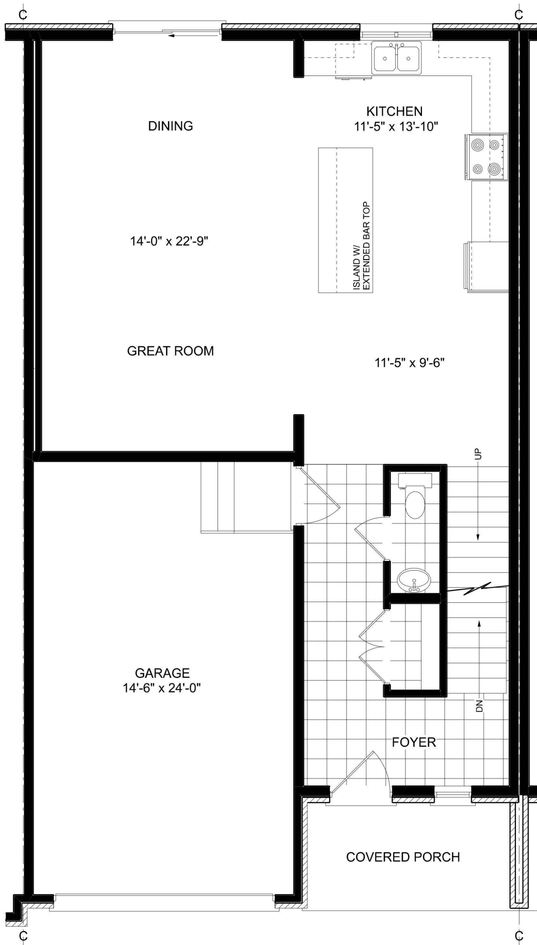
INTERIOR UNIT MAIN FLOOR PLAN 900 SQ.FT.
