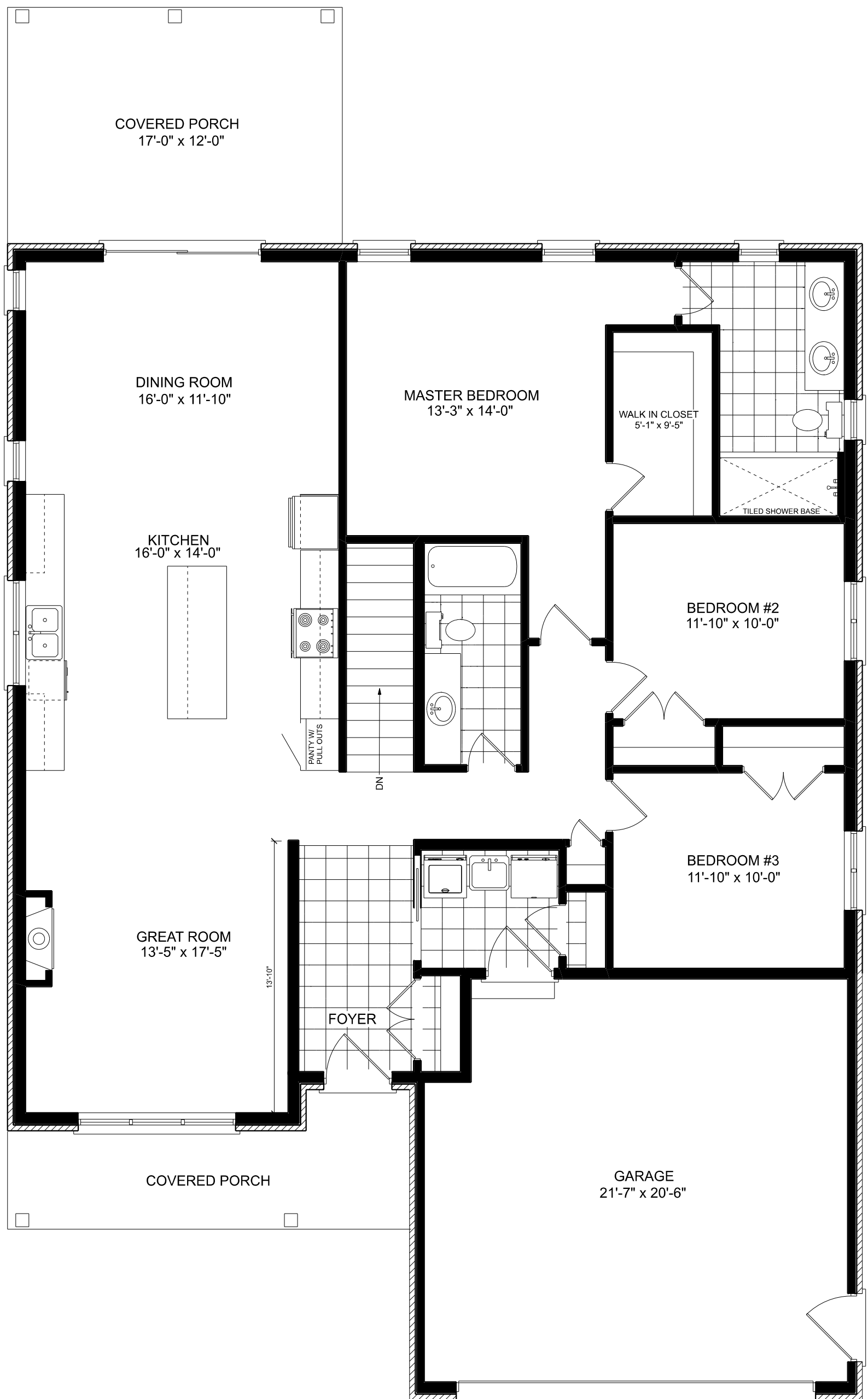
MAIN FLOOR PLAN 1785 SQ.FT. THE ASH
