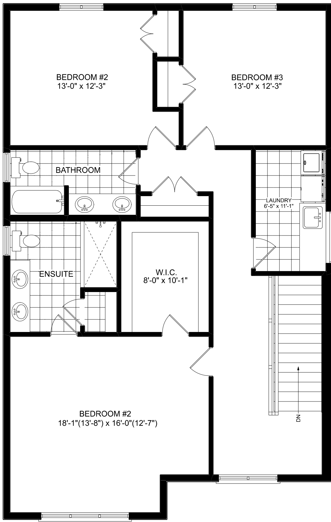
UPPER FLOOR PLAN 1300 SQ.FT.
