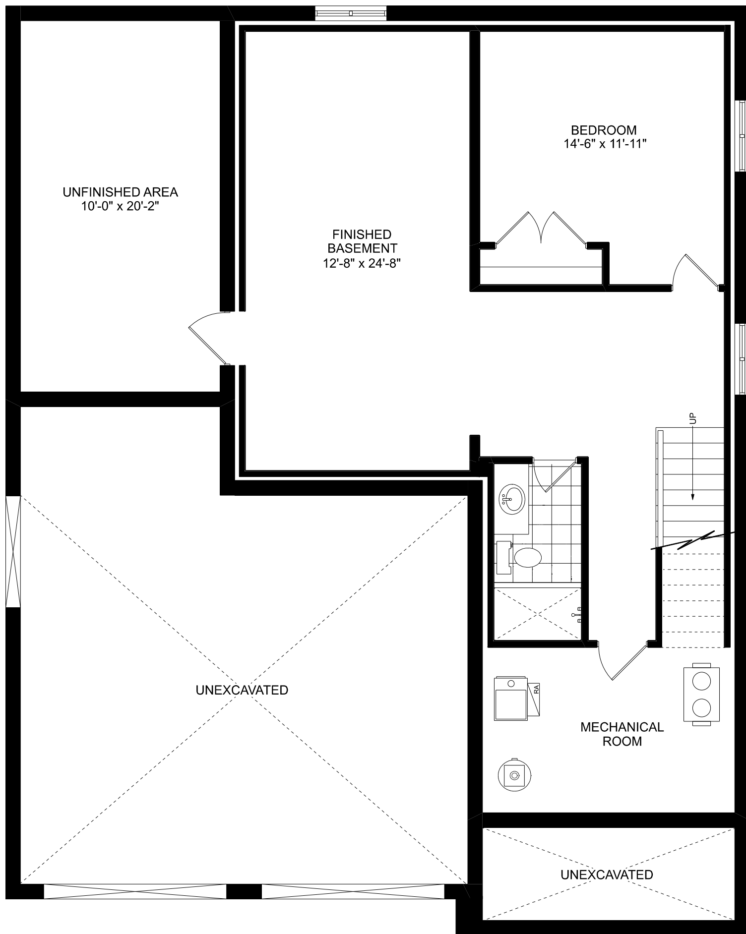
FOUNDATION PLAN FINISHED AREA = 778 SQ.FT.
