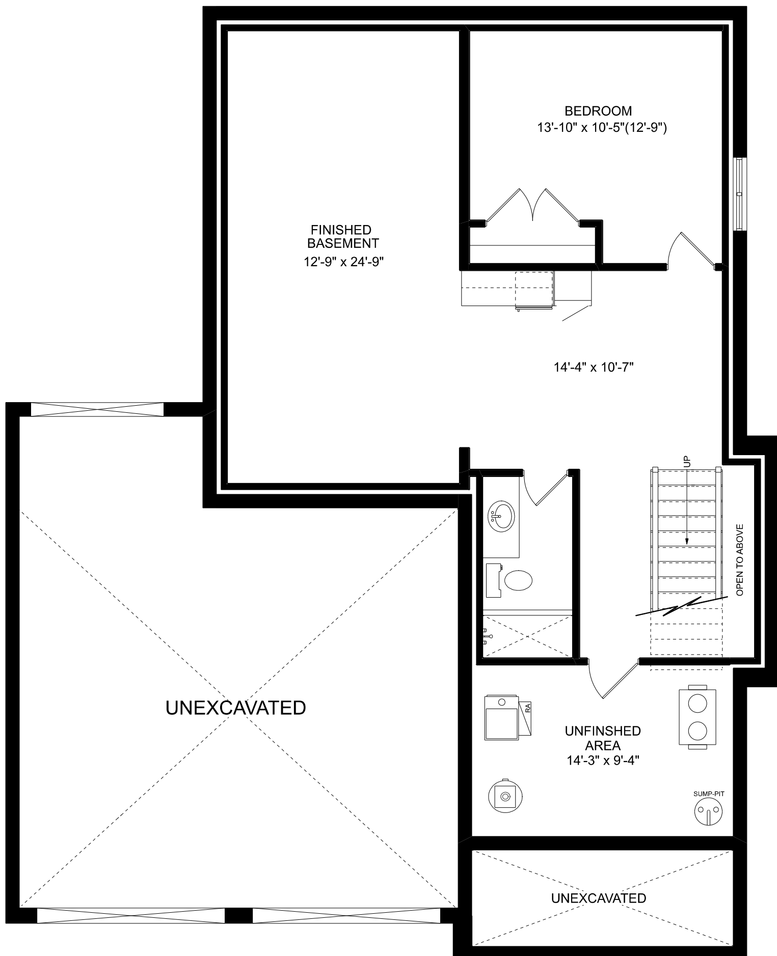
BASEMENT PLAN FINISHED AREA = 855 SQ.FT.
