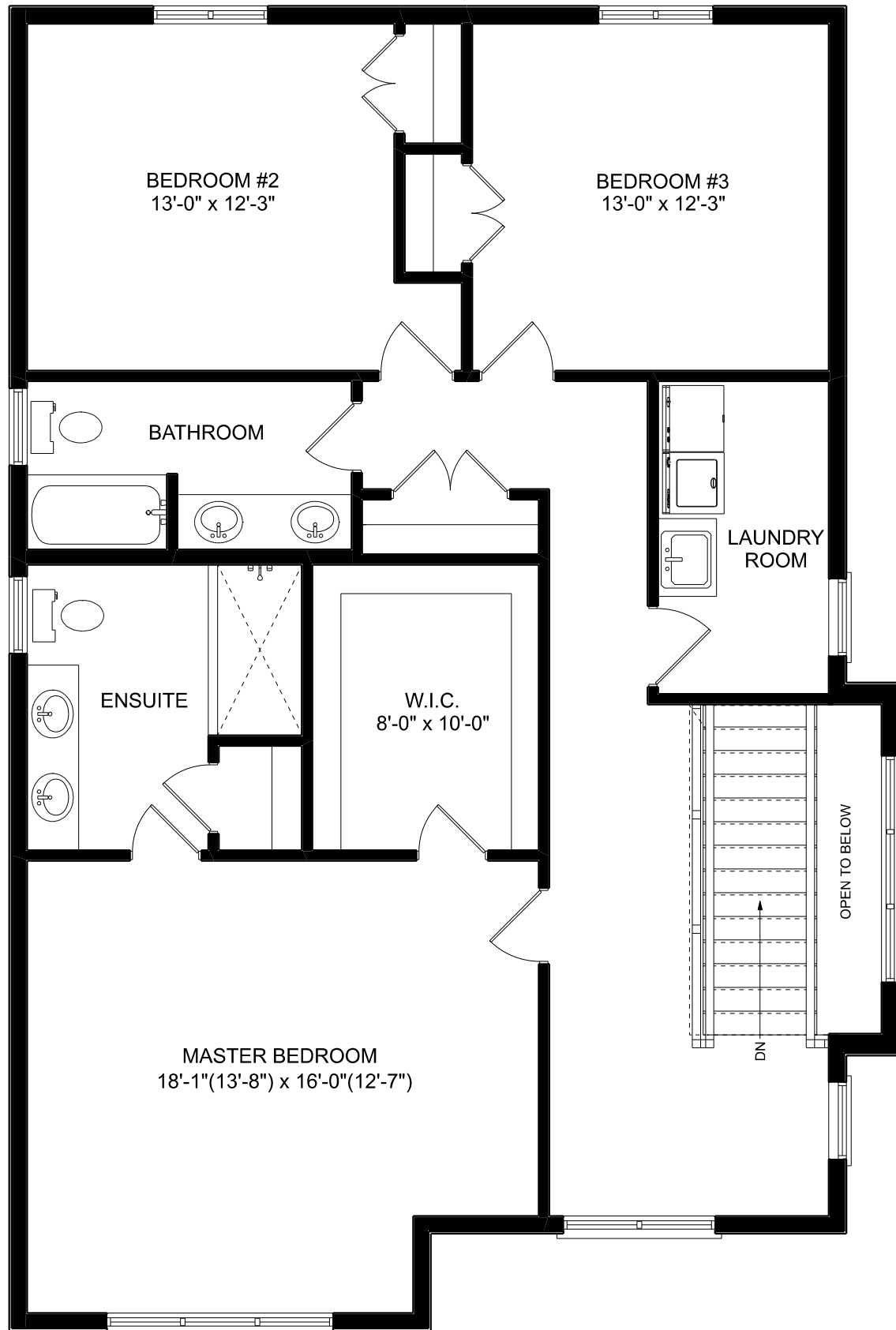
UPPER FLOOR PLAN 1300 SQ.FT.
