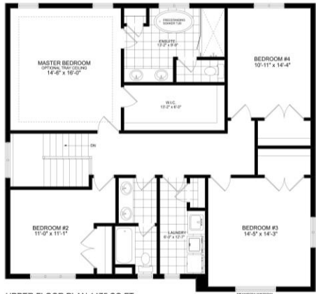
UPPER FLOOR PLAN 1475 SQ.FT. THE SYCAMORE
