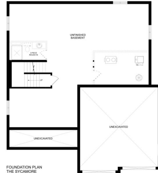
FOUNDATION PLAN THE SYCAMORE
