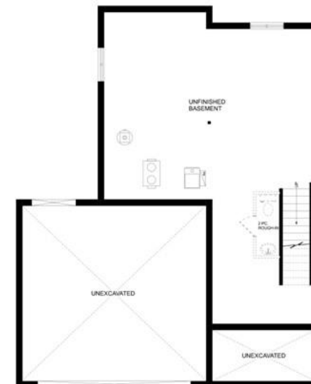
FOUNDATION PLAN THE SPRUCE
