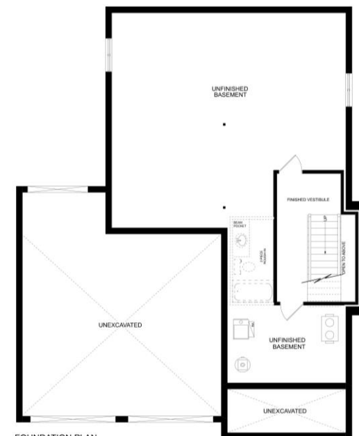
FOUNDATION PLAN THE MAGNOLIA
