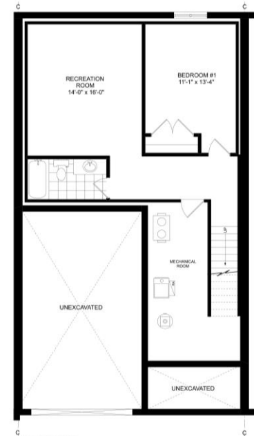
INTERIOR UNIT #11 OPTIONAL FINISHED BASEMENT PLAN - 585 SQ.FT.
