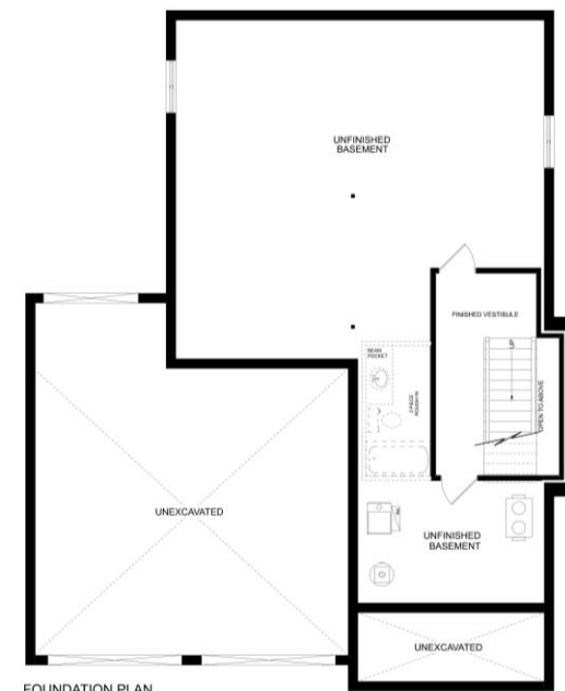
FOUNDATION PLAN
