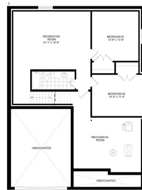
EXTERIOR UNIT #13 OPTIONAL FINISHED BASEMENT PLAN - 900 SQ.FT.
