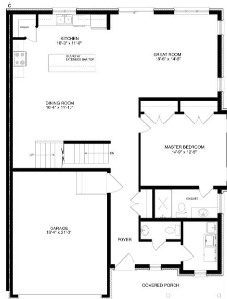
EXTERIOR UNIT #13 MAIN FLOOR PLAN 1403 SQ.FT.
