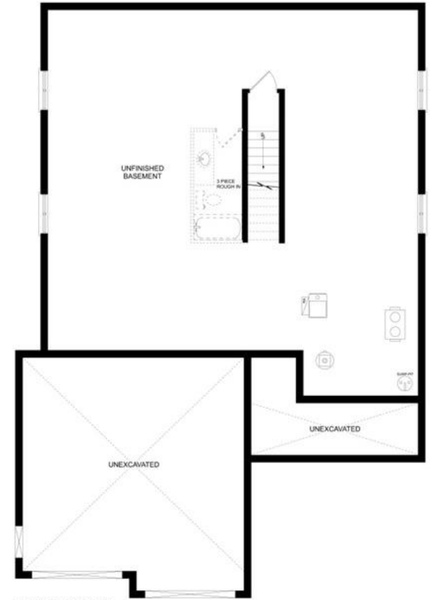
FOUNDATION PLAN
