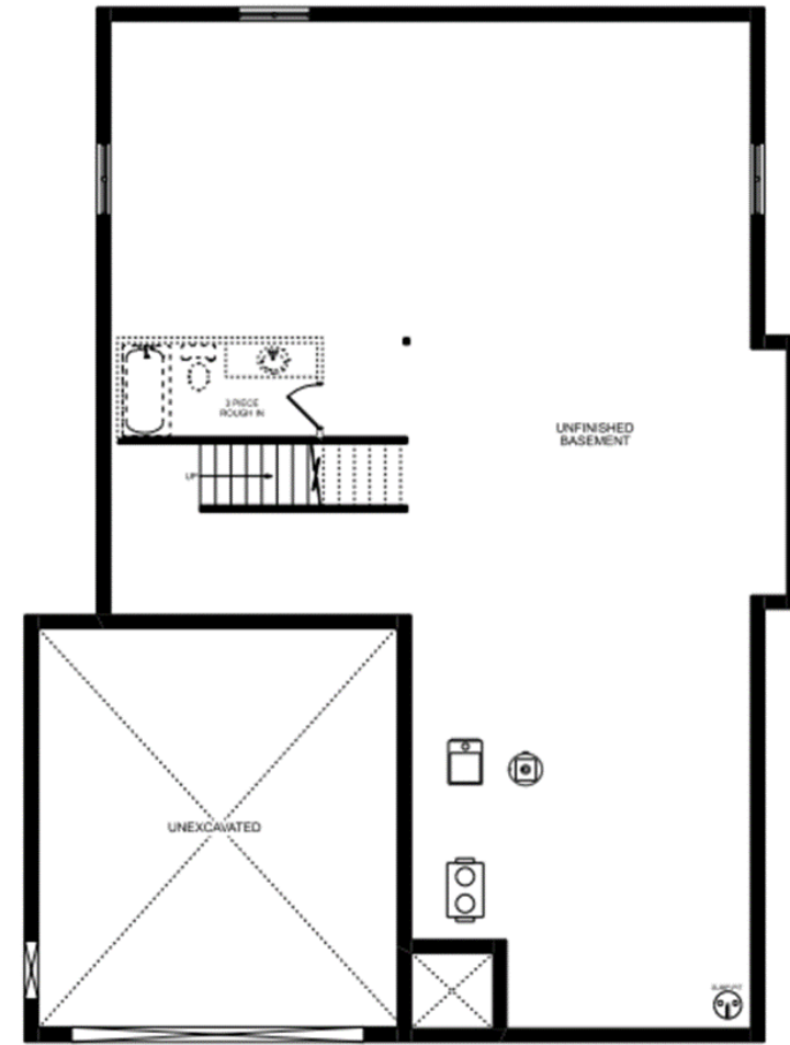
FOUNDATION PLAN
