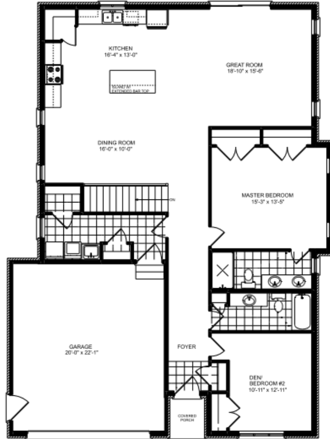
MAIN FLOOR PLAN 1745 SQ.FT. THE CEDAR
