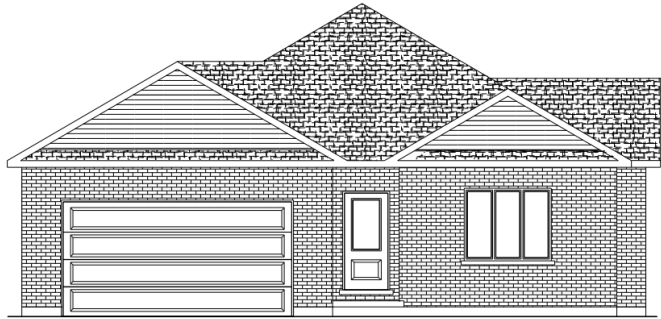
FRONT ELEVATION 'A' THE CEDAR
