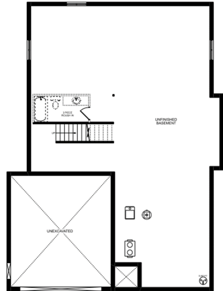
FOUNDATION PLAN THE CEDAR
