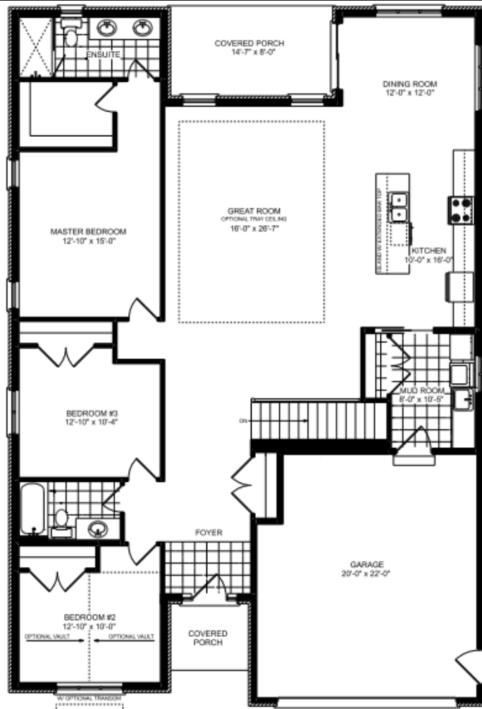
MAIN FLOOR PLAN 2010 SQ.FT. THE BALSAM
