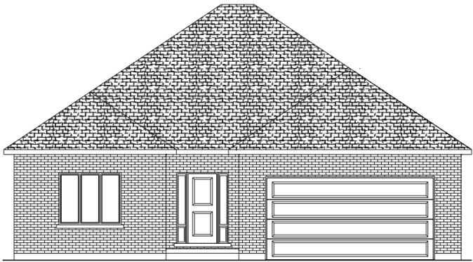
FRONT ELEVATION 'A' THE BALSAM
