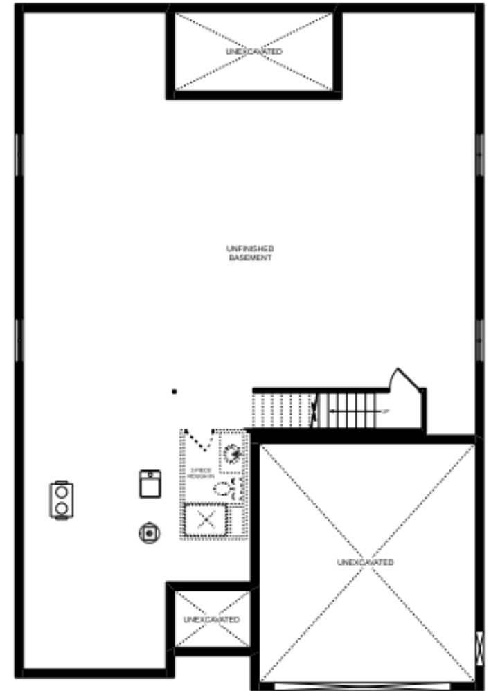
BASEMENT PLAN THE BALSAM
