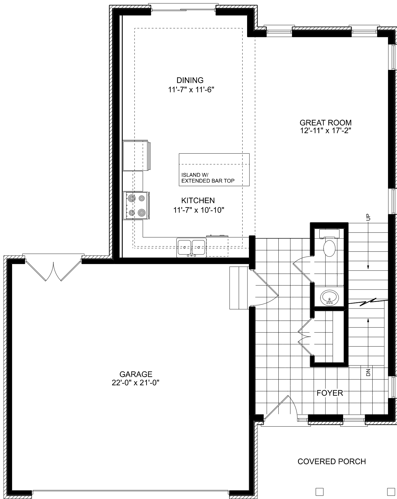
MAIN FLOOR PLAN 815 SQ.FT. THE SPRUCE
