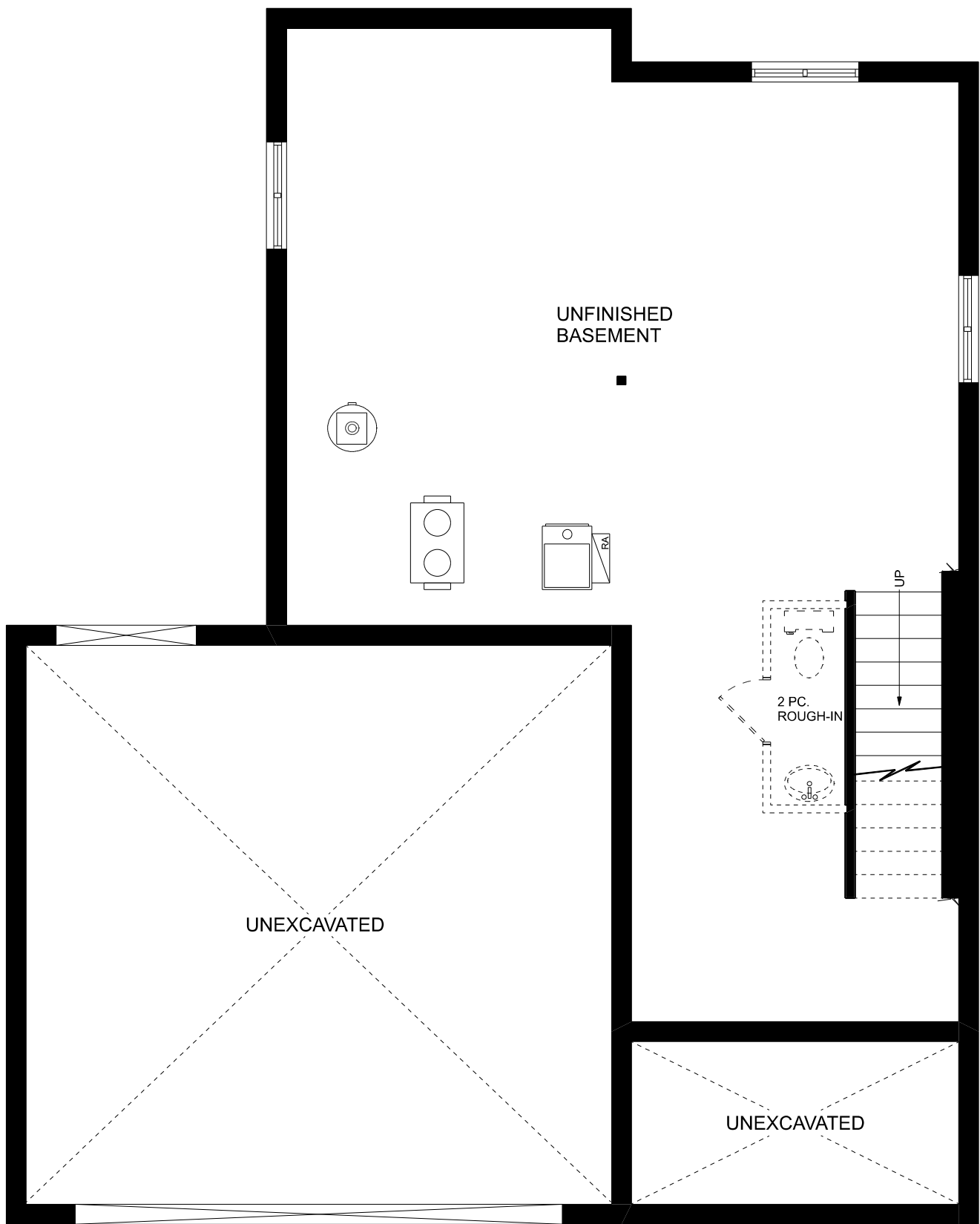
FOUNDATION PLAN THE SPRUCE
