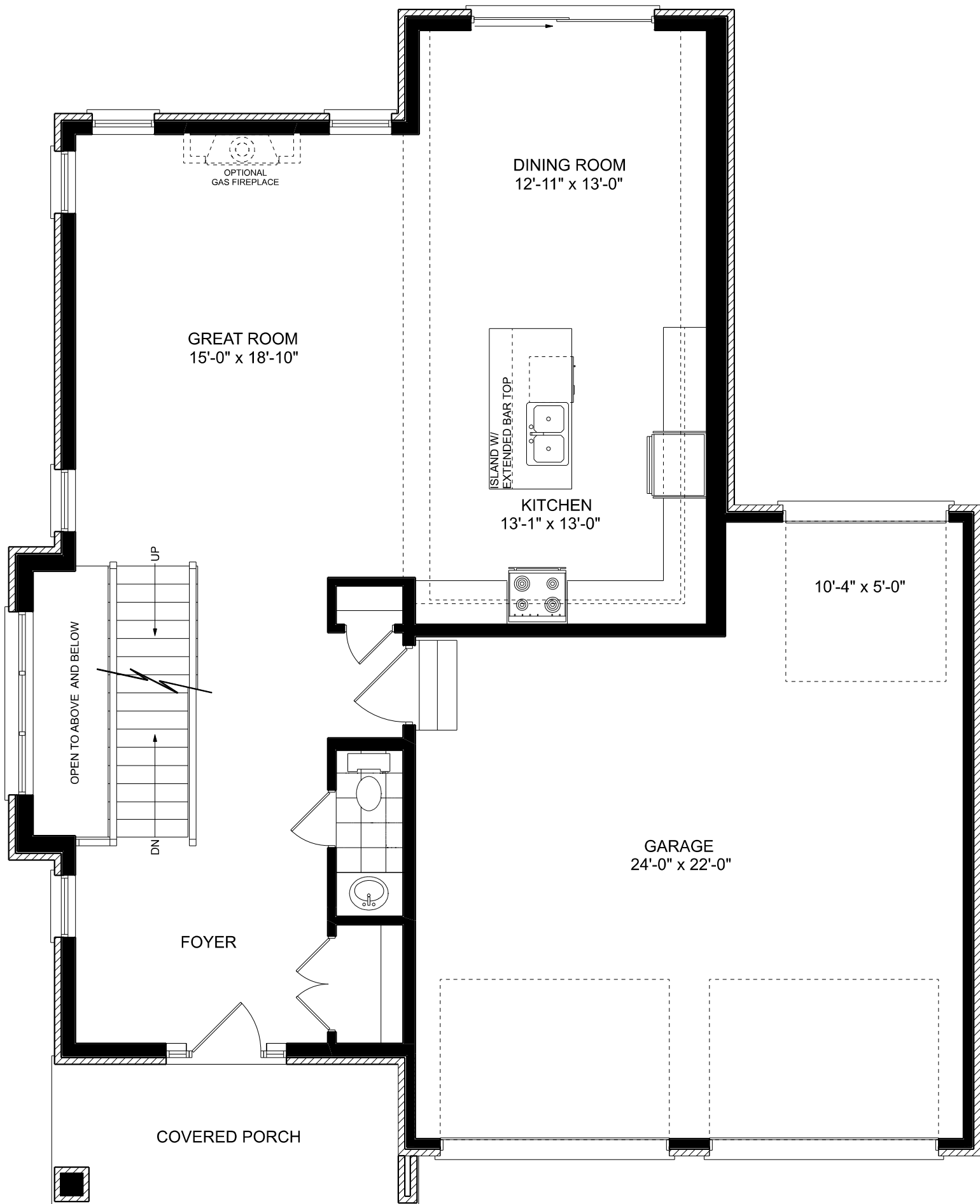
MAIN FLOOR PLAN 1010 SQ.FT. THE MAGNOLIA
