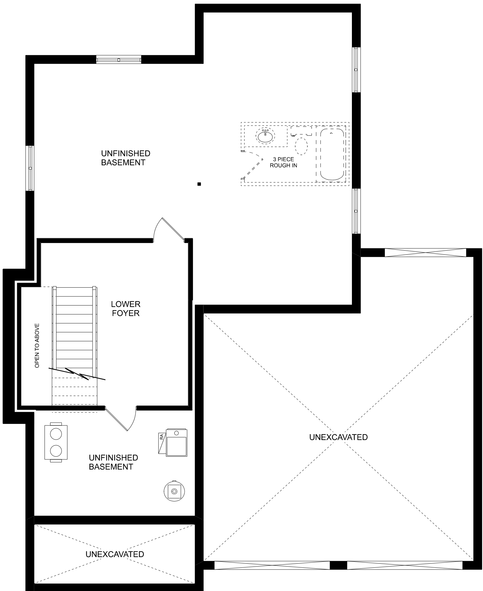
FOUNDATION PLAN THE MAGNOLIA
