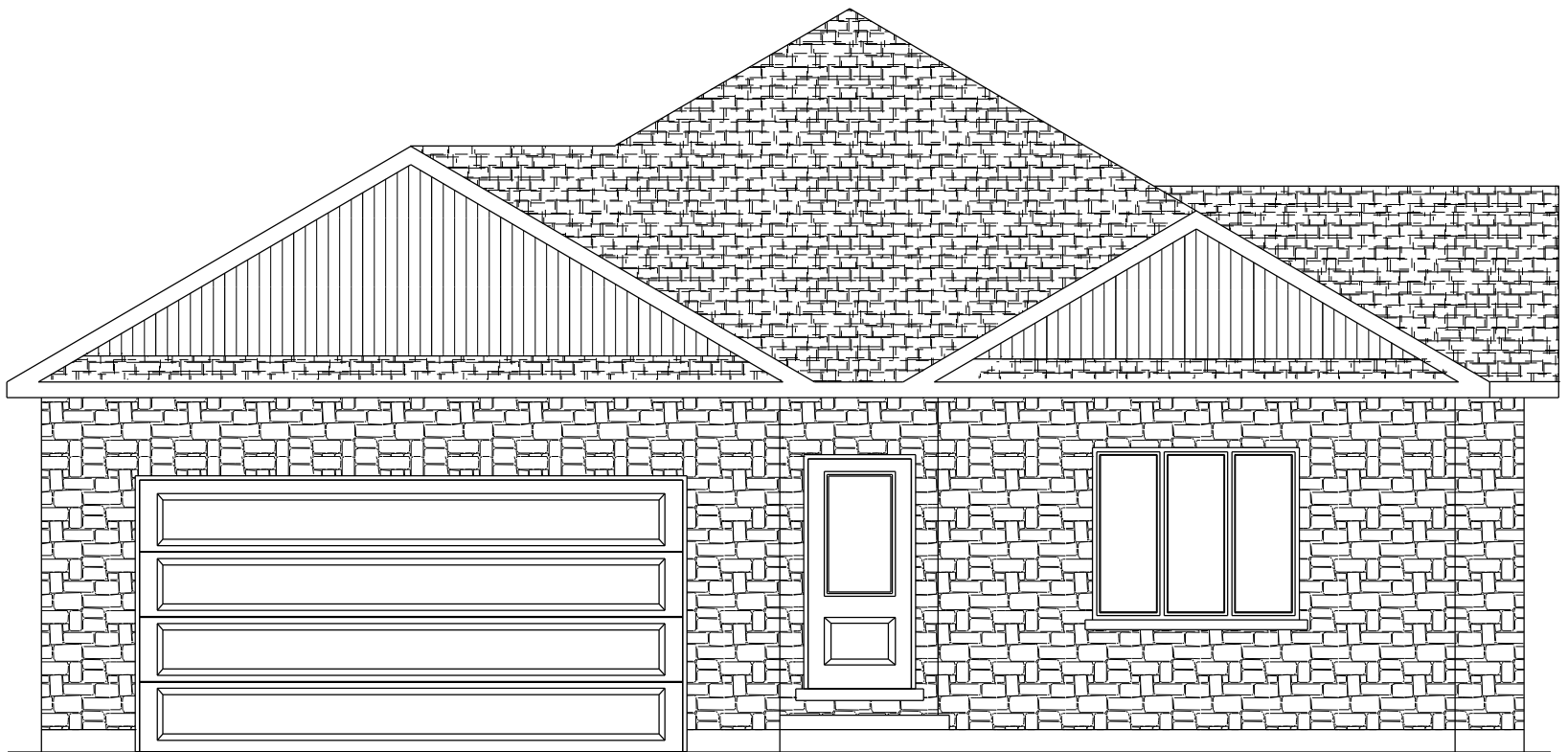
FRONT ELEVATION 'B' THE CEDAR
