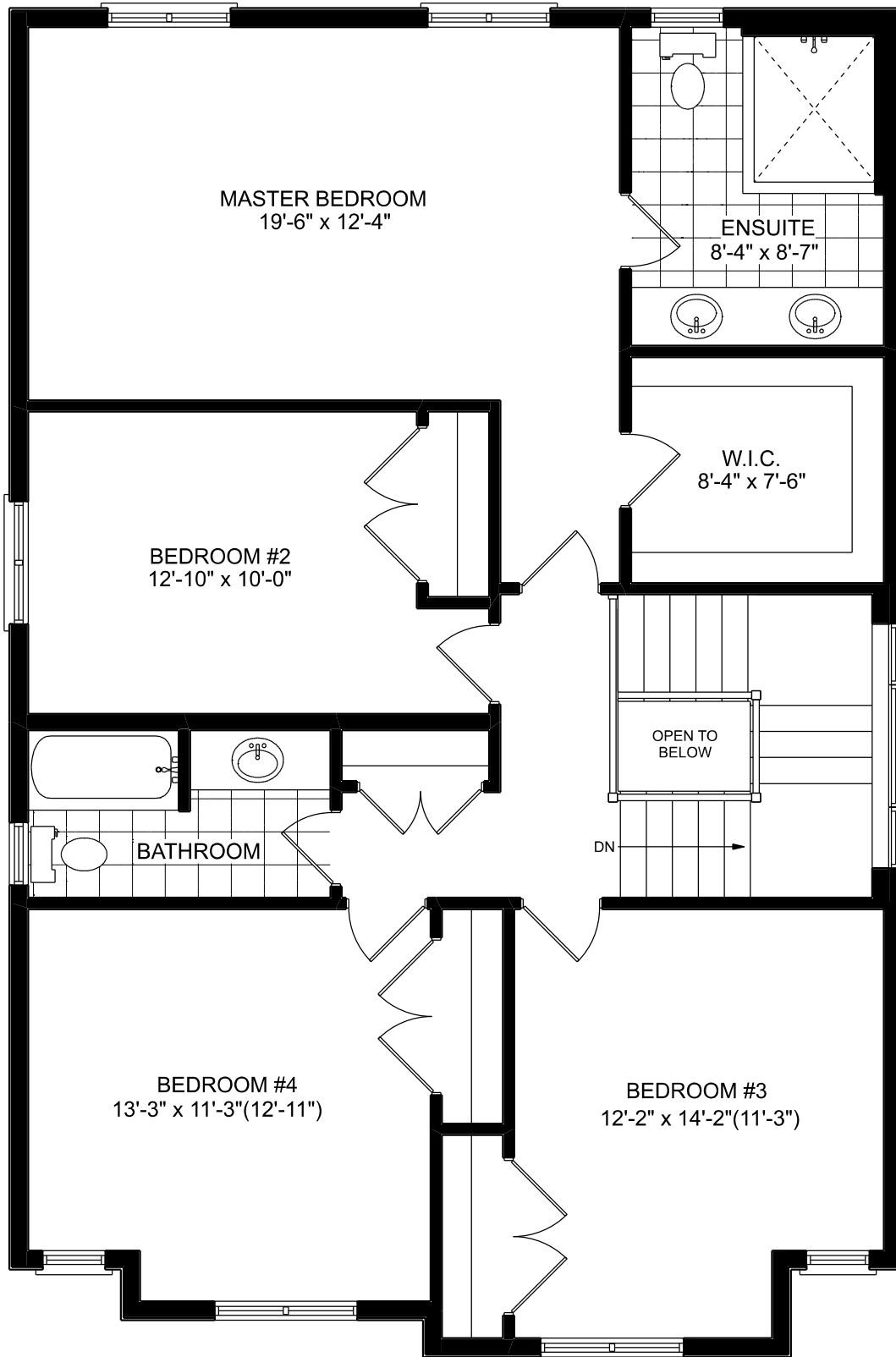
UPPER FLOOR PLAN 1250 SQ.FT. THE WESTMOUNT
