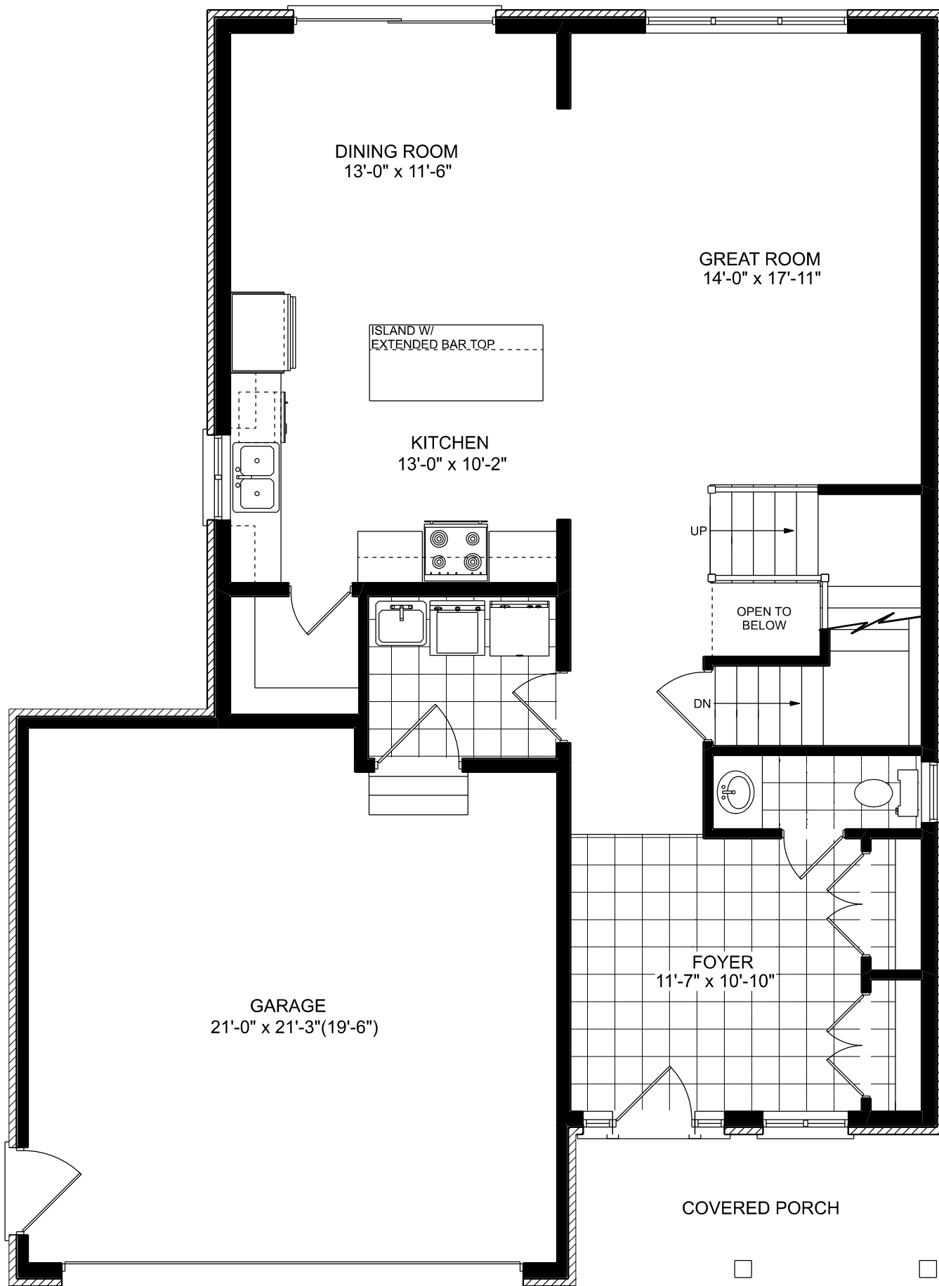
MAIN FLOOR PLAN 1090 SQ.FT. THE WESTMOUNT
