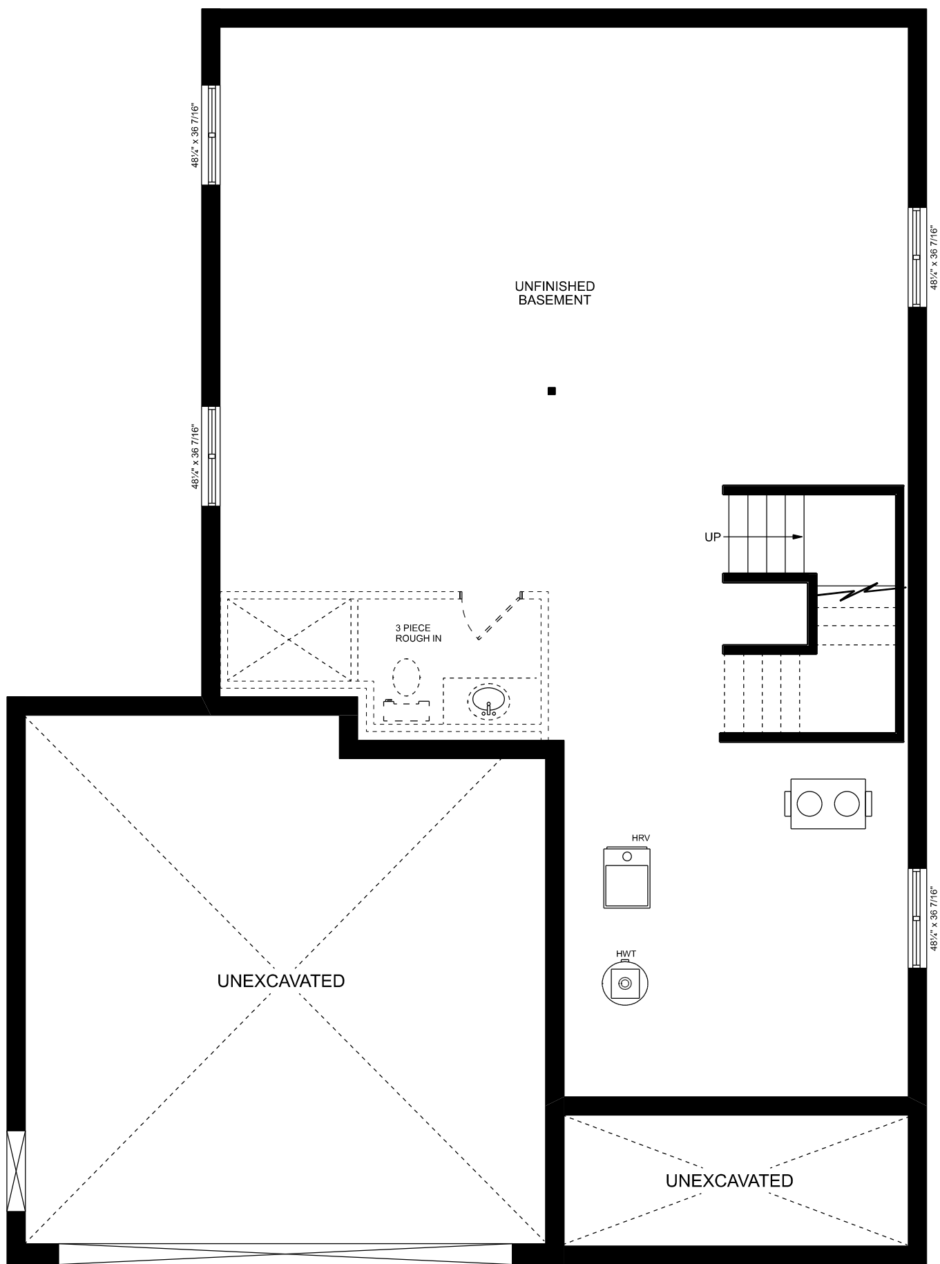
FOUNDATION PLAN THE WESTMOUNT
